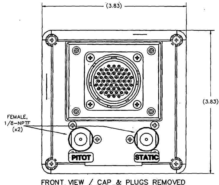
FRONT VIEW / CAP & PLUGS REMOVED
